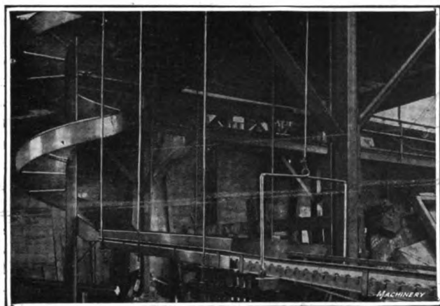
Fig. 36—For unloading flywheel castings from freight cars, the Cadillac Motor Car Co., of Detroit, Mich., has a spiral steel chute leading down from the platform on which the load is discharged. The castings are ejected from the chute onto a gravity carrier
